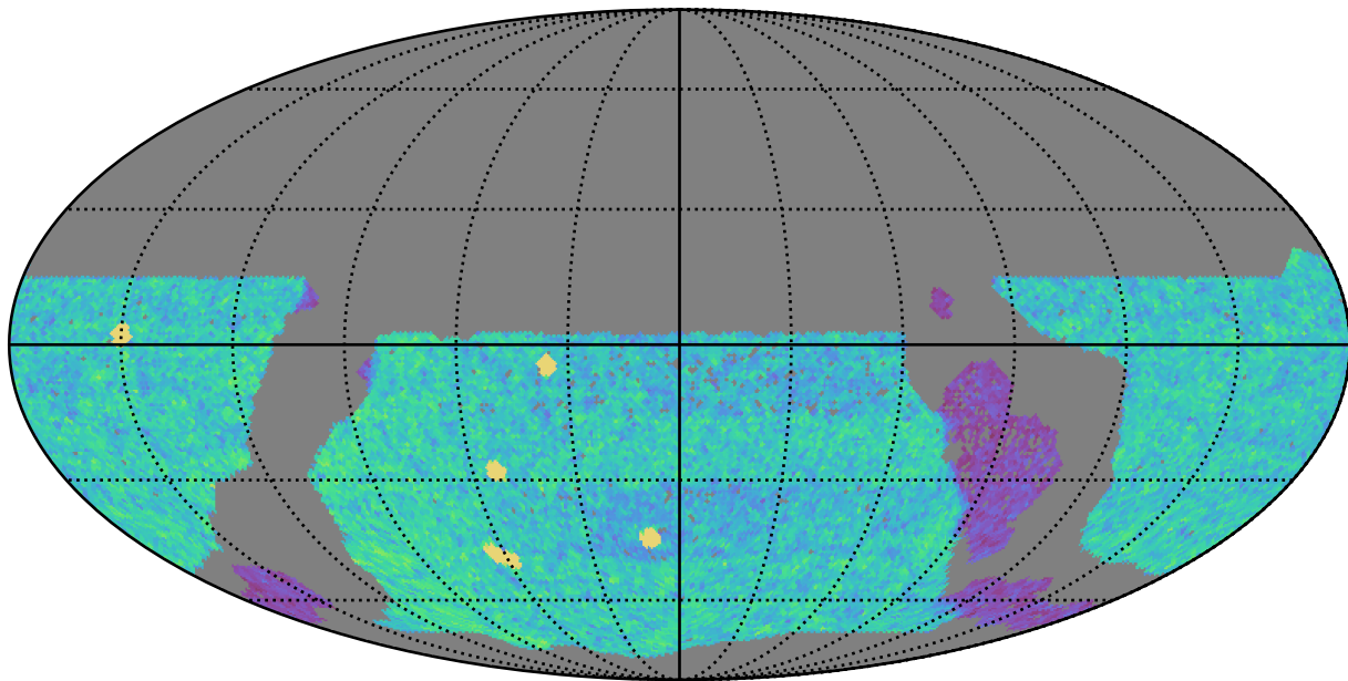
too_10_1v3.4_10yrs WFD u band: NVisits
