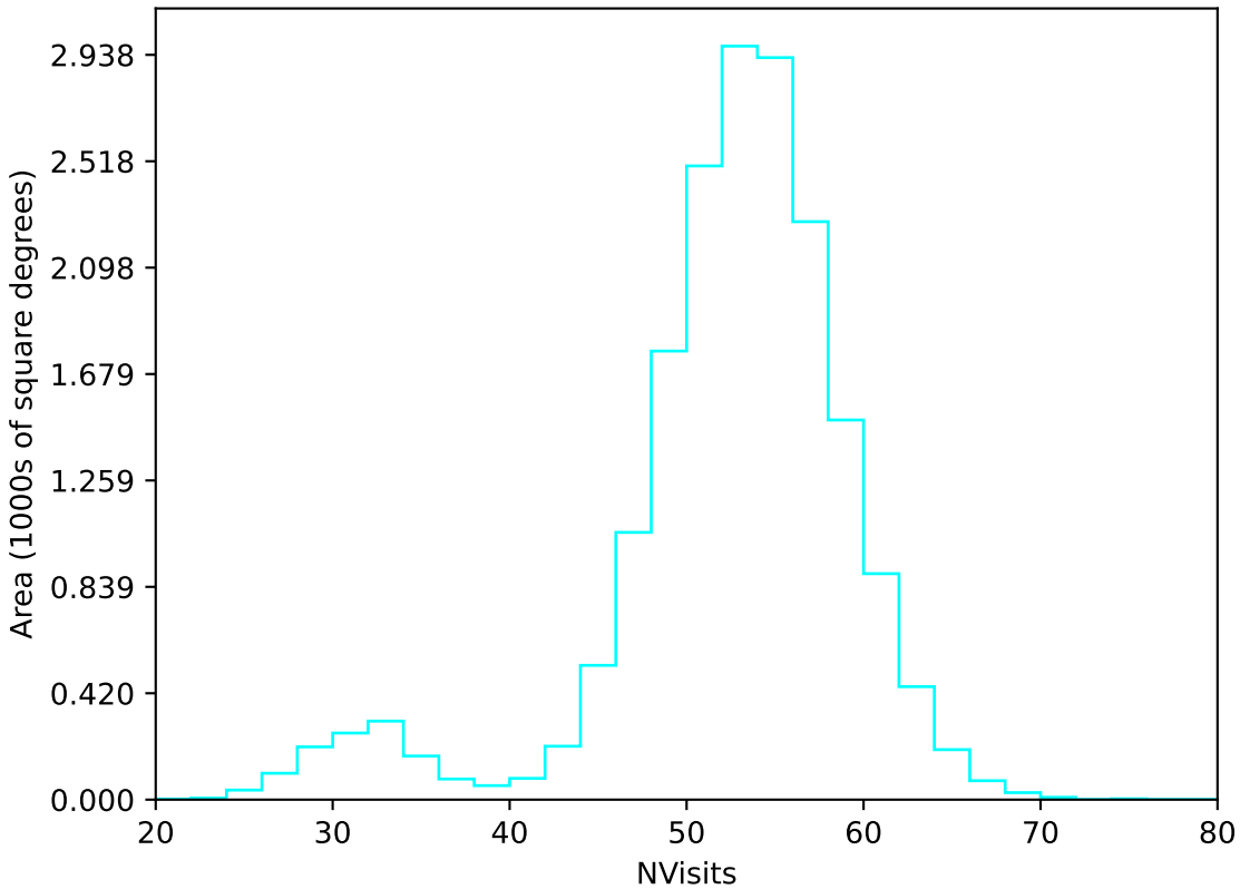
too_10_1v3.4_10yrs WFD u band: NVisits
