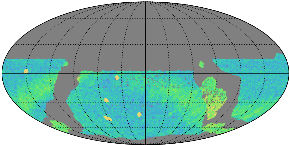
too_10_1v3.4_10yrs WFD r band: NVisits
