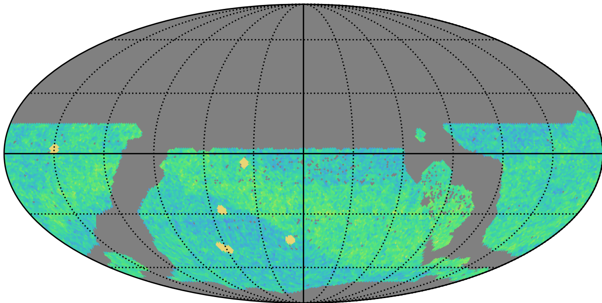
too_10_1v3.4_10yrs WFD i band: NVisits
