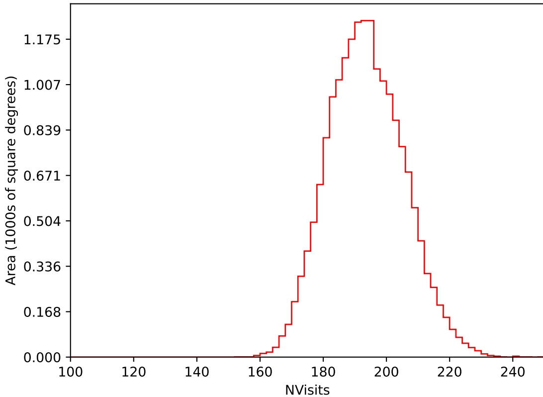
too_10_1v3.4_10yrs WFD i band: NVisits
