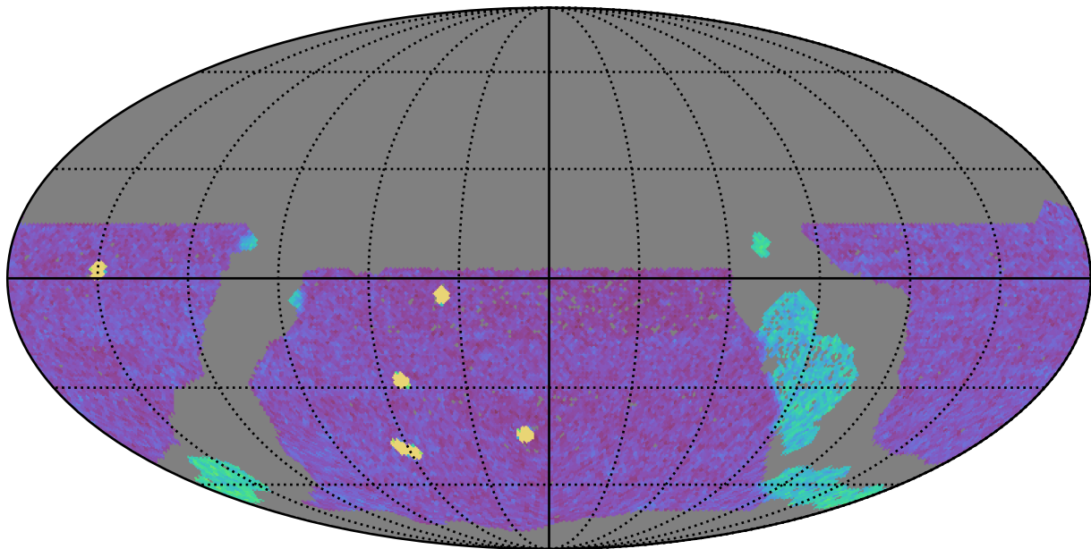
too_10_1v3.4_10yrs WFD g band: NVisits
