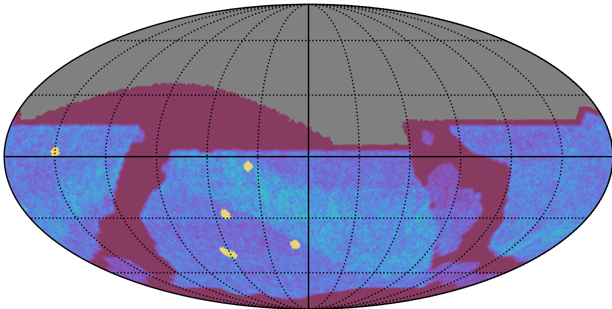
too_10_1v3.4_10yrs All sky z band: NVisits
