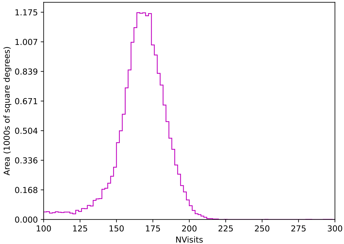
too_10_1v3.4_10yrs All sky z band: NVisits
