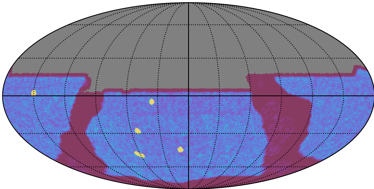
too_10_1v3.4_10yrs All sky y band: NVisits
