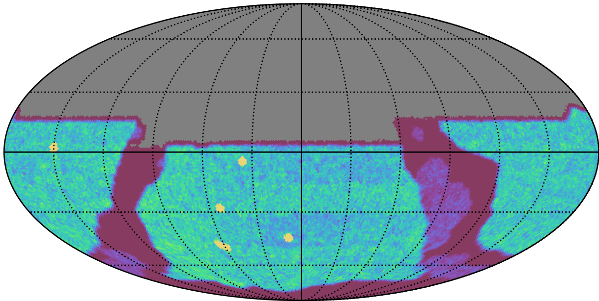
too_10_1v3.4_10yrs All sky u band: NVisits
