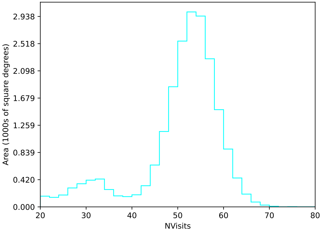
too_10_1v3.4_10yrs All sky u band: NVisits
