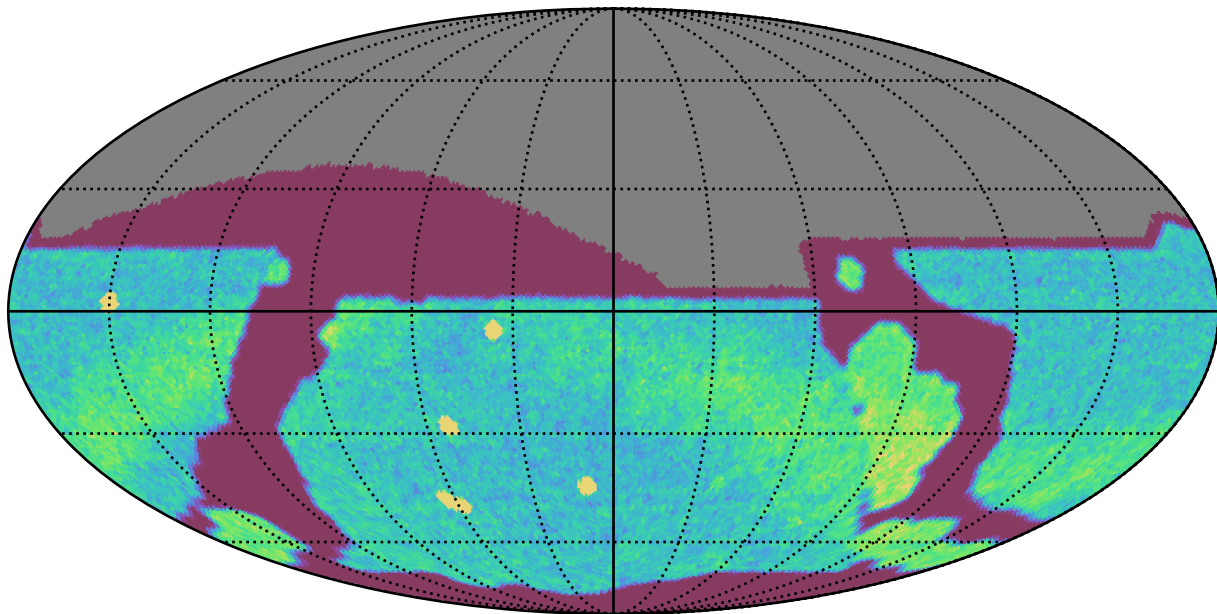
too_10_1v3.4_10yrs All sky r band: NVisits
