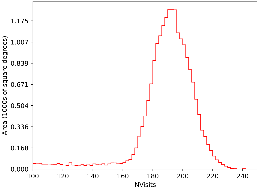
too_10_1v3.4_10yrs All sky i band: NVisits
