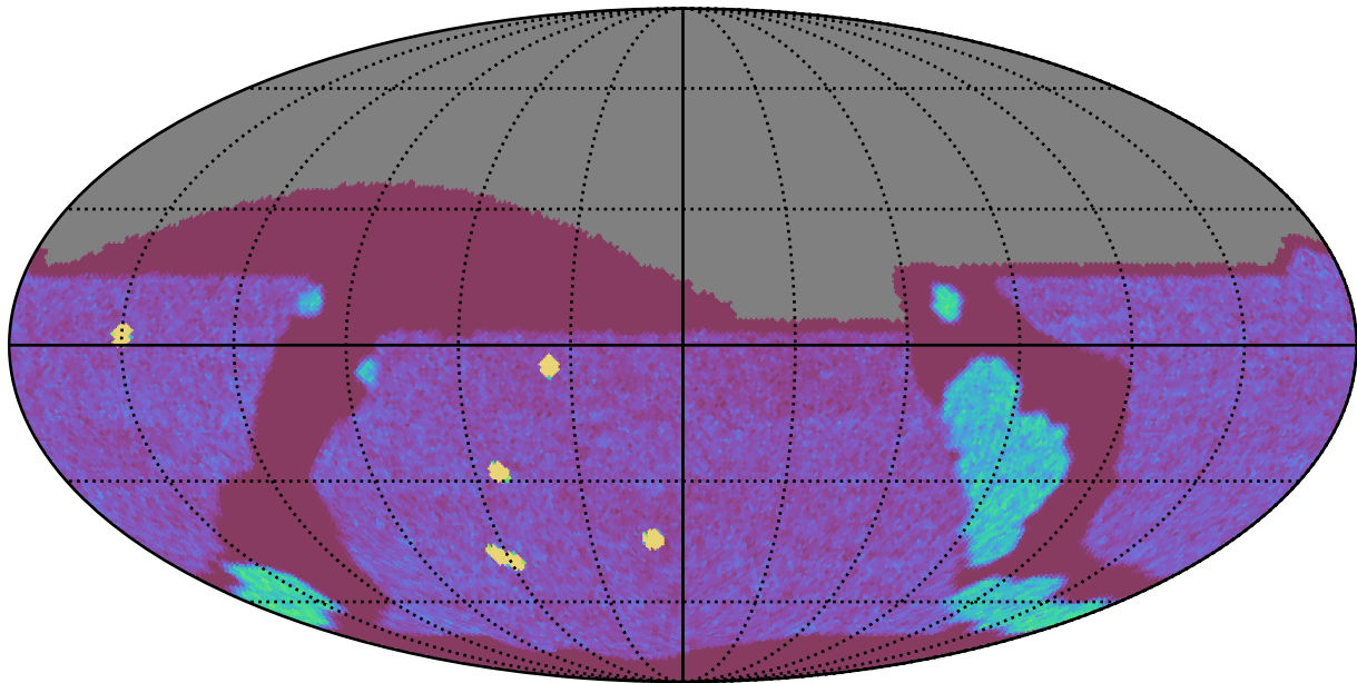
too_10_1v3.4_10yrs All sky g band: NVisits
