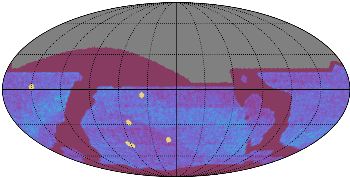
too_10_1v3.4_10yrs All sky all bands: NVisits
