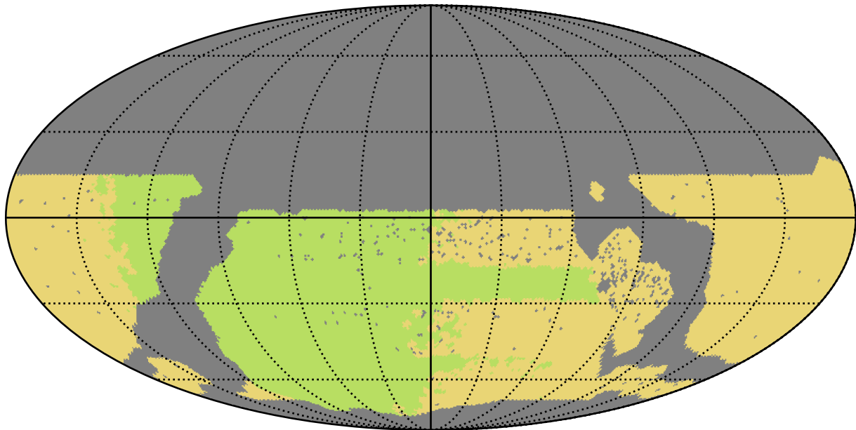
too_10_1v3.4_10yrs WFD all bands: NSeasons
