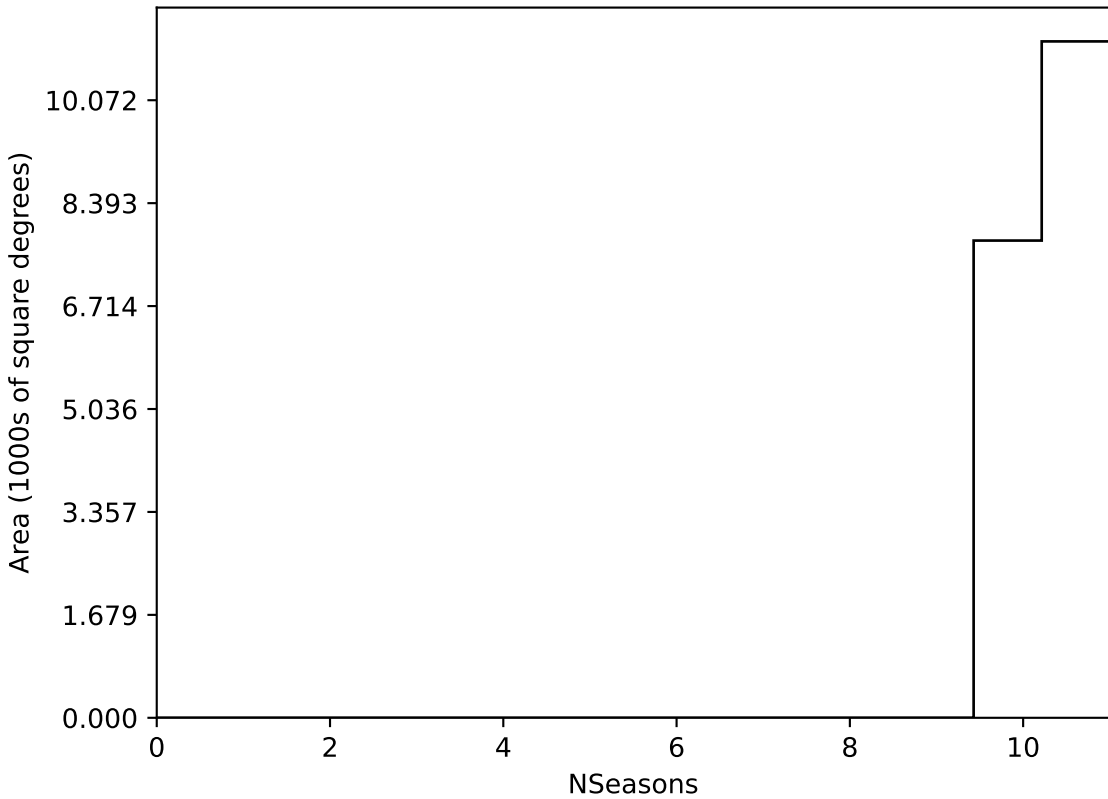
too_10_1v3.4_10yrs WFD all bands: NSeasons
