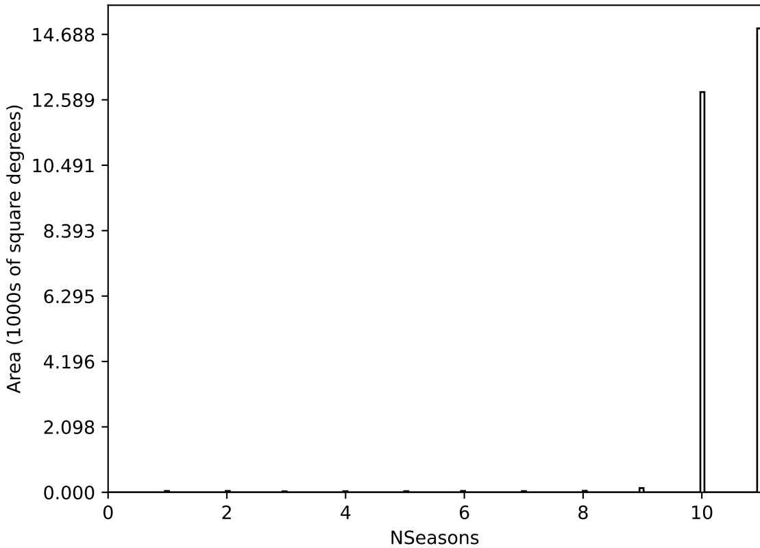
too_10_1v3.4_10yrs All sky all bands: NSeasons
