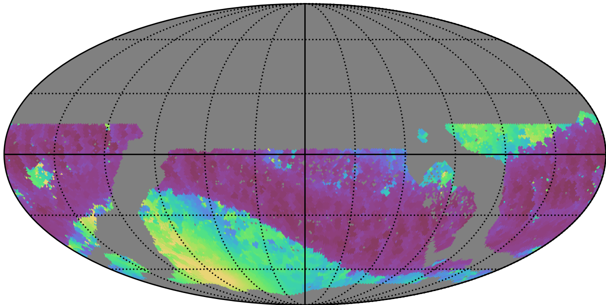
too_10_1v3.4_10yrs WFD z band: Min solarElong
