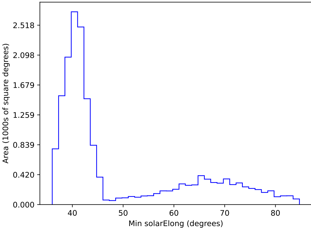
too_10_1v3.4_10yrs WFD z band: Min solarElong
