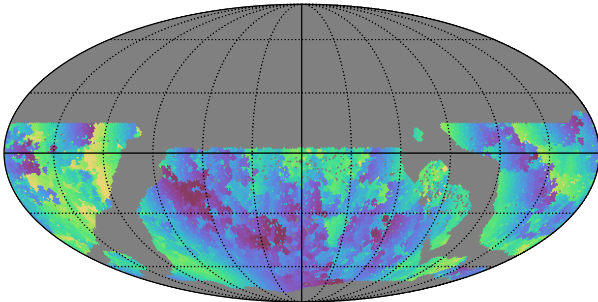
too_10_1v3.4_10yrs WFD u band: Min solarElong
