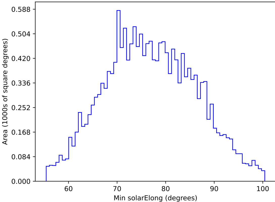
too_10_1v3.4_10yrs WFD u band: Min solarElong
