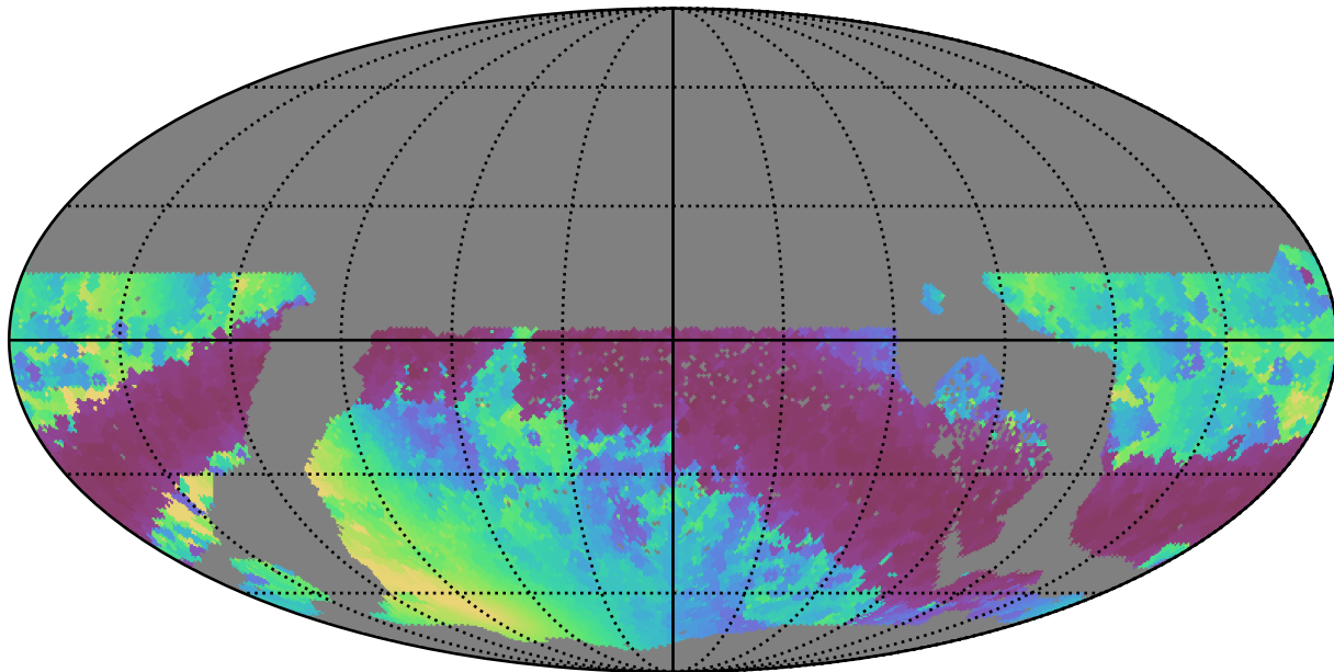
too_10_1v3.4_10yrs WFD r band: Min solarElong
