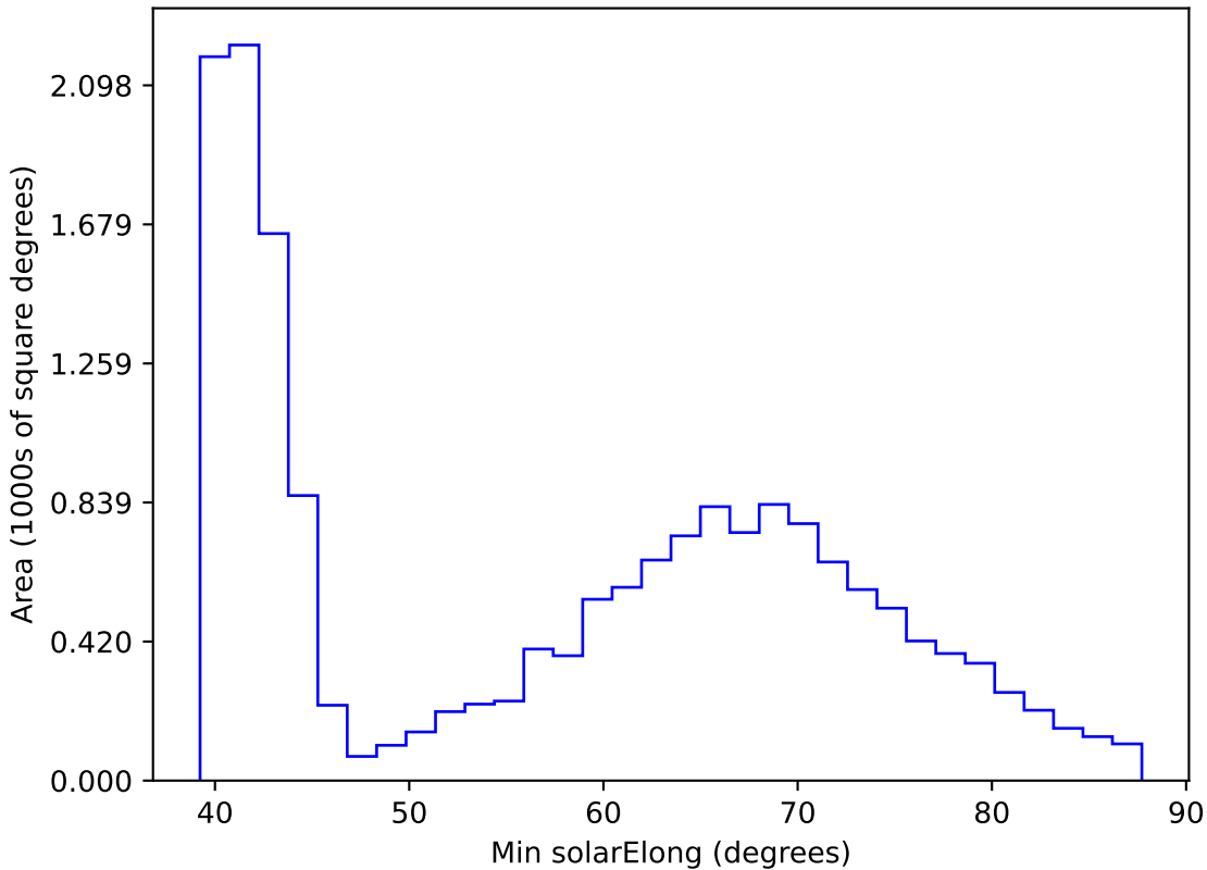
too_10_1v3.4_10yrs WFD r band: Min solarElong
