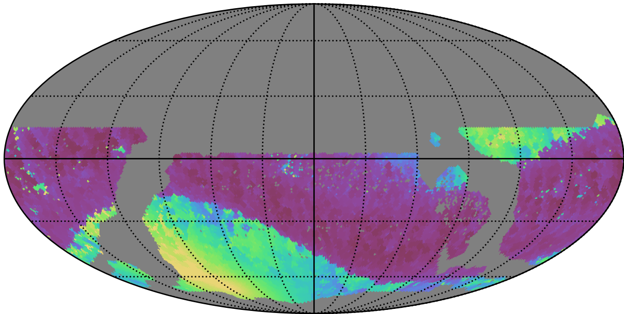
too_10_1v3.4_10yrs WFD i band: Min solarElong
