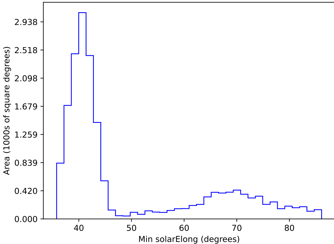
too_10_1v3.4_10yrs WFD i band: Min solarElong
