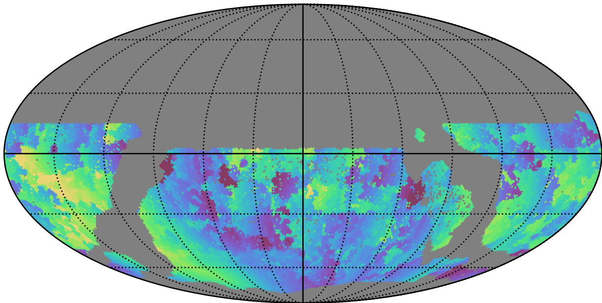
too_10_1v3.4_10yrs WFD g band: Min solarElong
