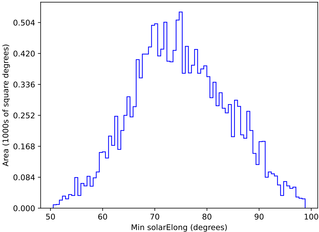
too_10_1v3.4_10yrs WFD g band: Min solarElong
