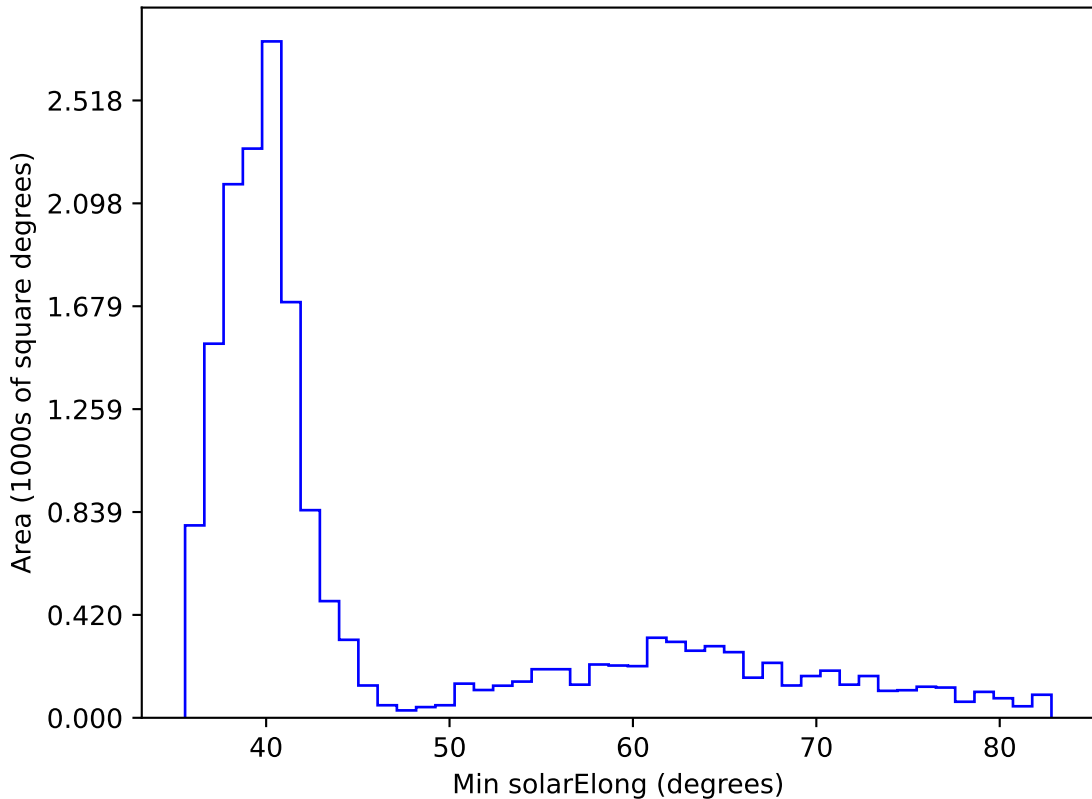
too_10_1v3.4_10yrs WFD all bands: Min solarElong
