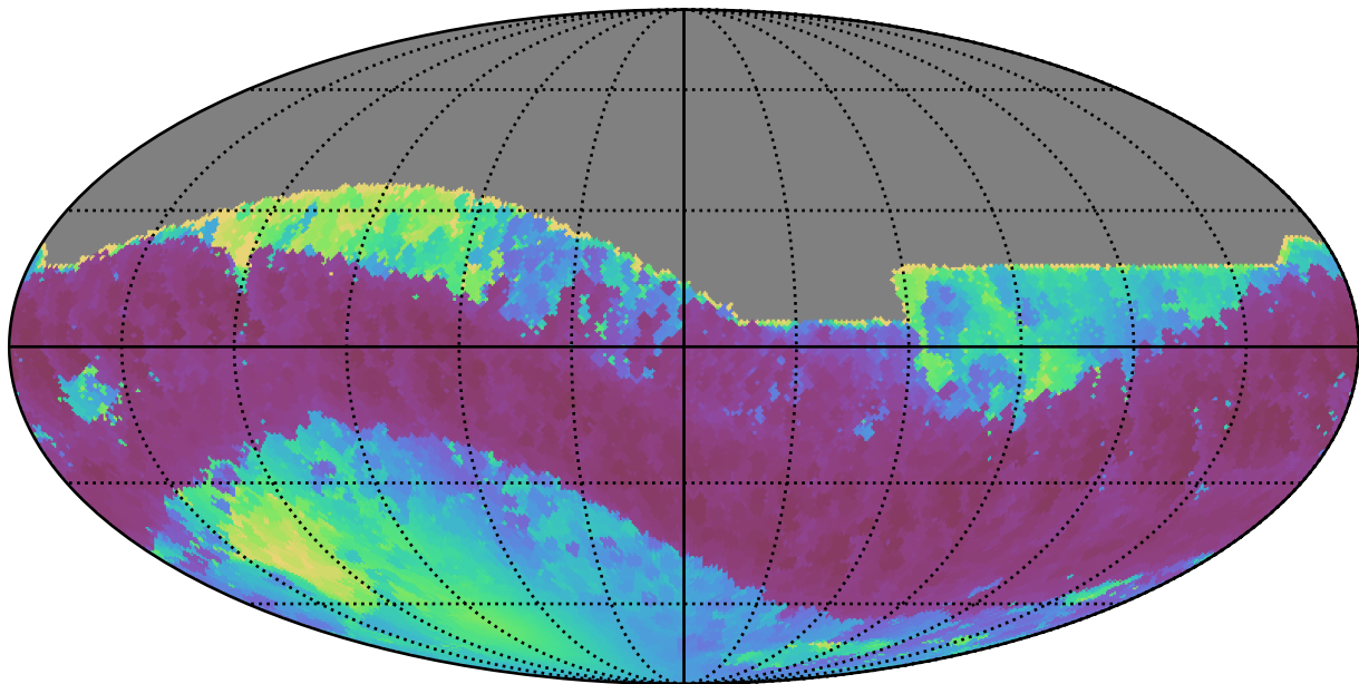
too_10_1v3.4_10yrs All sky z band: Min solarElong
