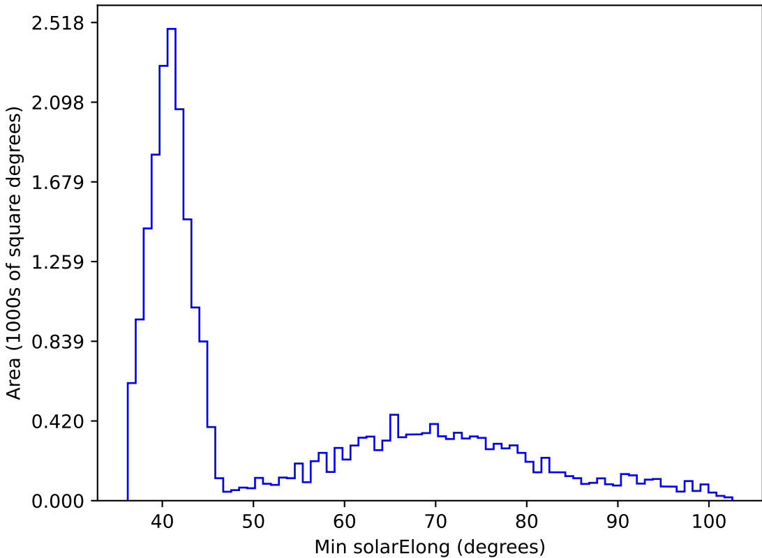
too_10_1v3.4_10yrs All sky z band: Min solarElong
