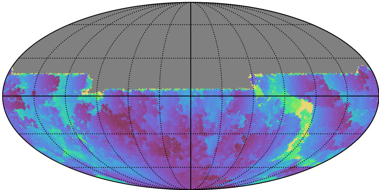
too_10_1v3.4_10yrs All sky u band: Min solarElong
