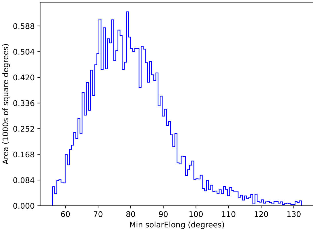
too_10_1v3.4_10yrs All sky u band: Min solarElong
