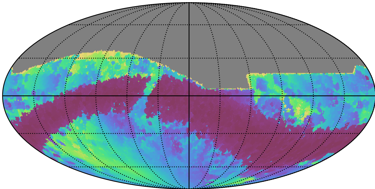
too_10_1v3.4_10yrs All sky r band: Min solarElong
