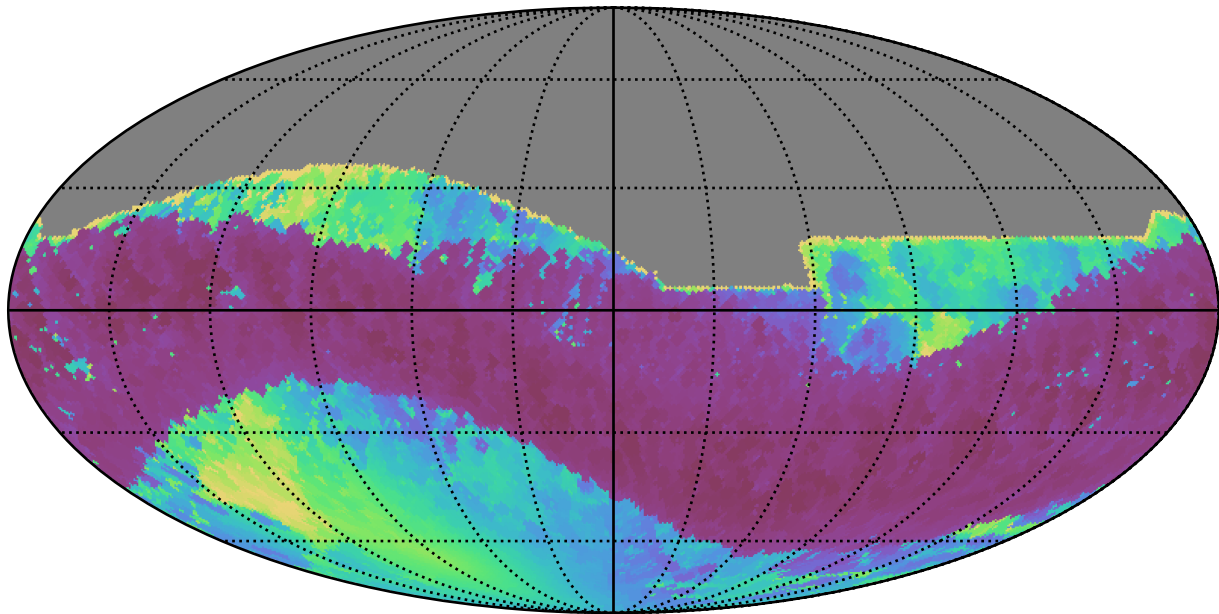
too_10_1v3.4_10yrs All sky i band: Min solarElong
