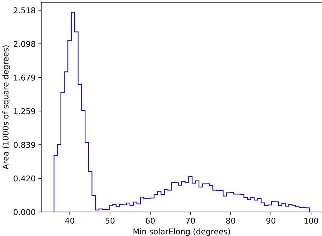
too_10_1v3.4_10yrs All sky i band: Min solarElong
