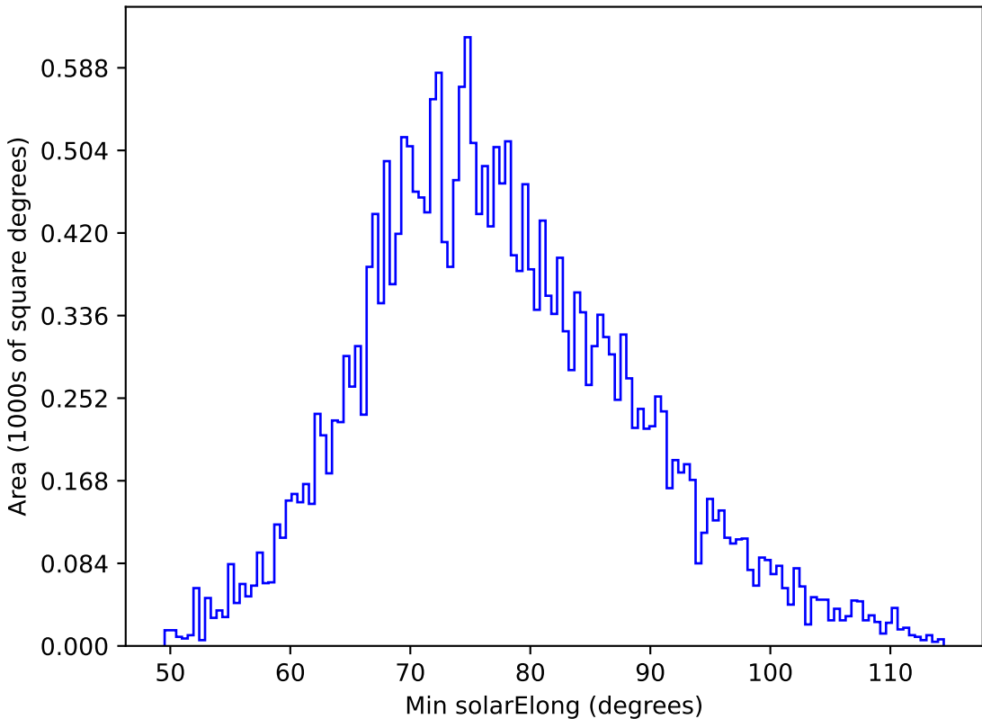
too_10_1v3.4_10yrs All sky g band: Min solarElong
