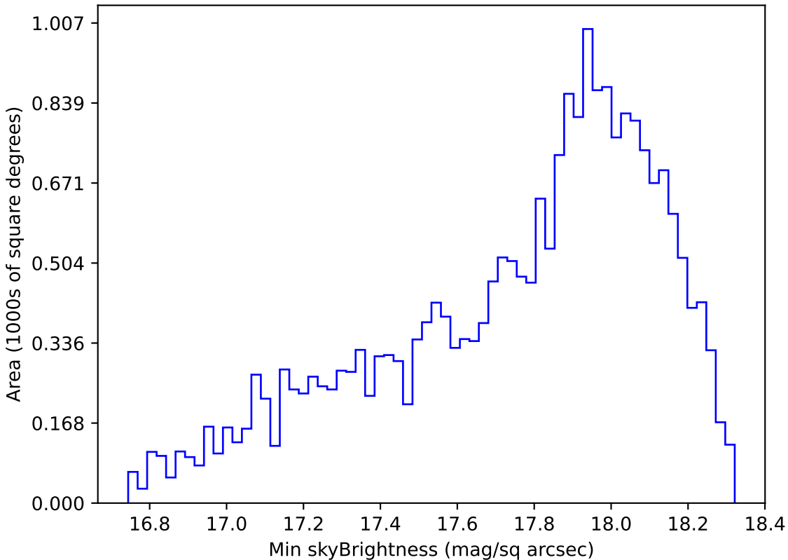
too_10_1v3.4_10yrs Yr 1 y band: Min skyBrightness
