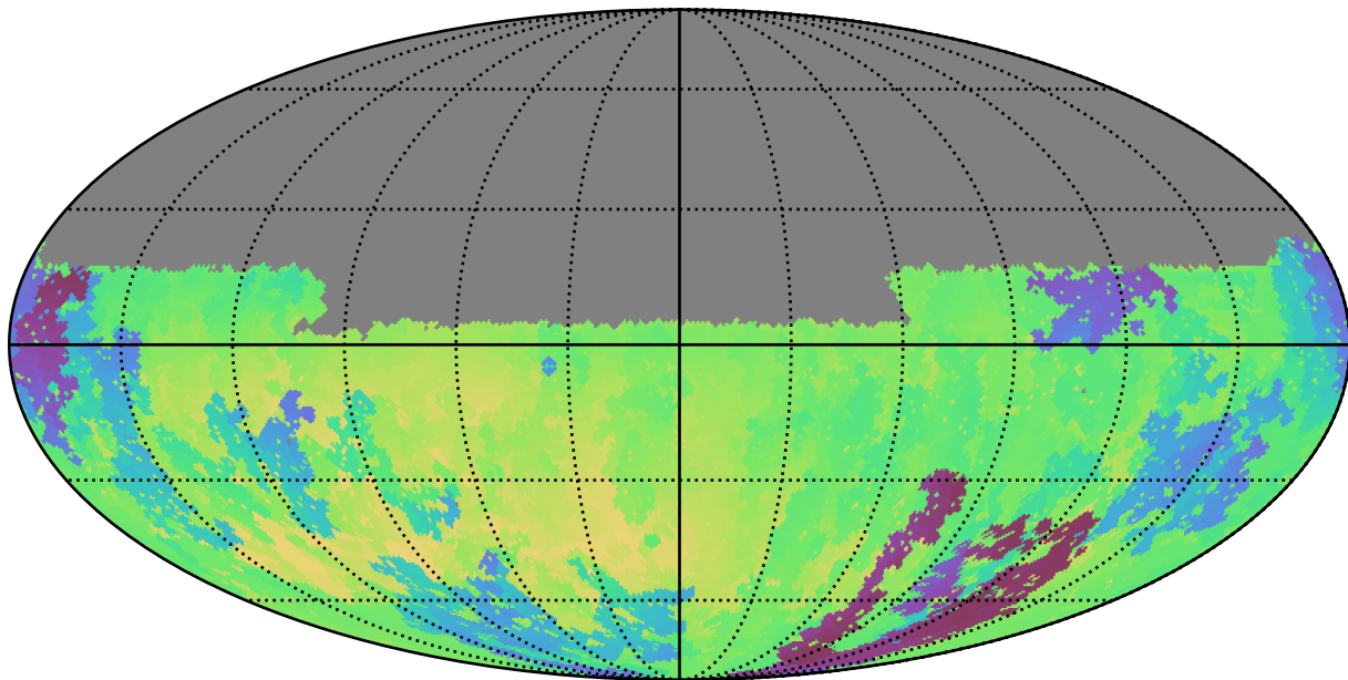
too_10_1v3.4_10yrs Yr 1 u band: Min skyBrightness
