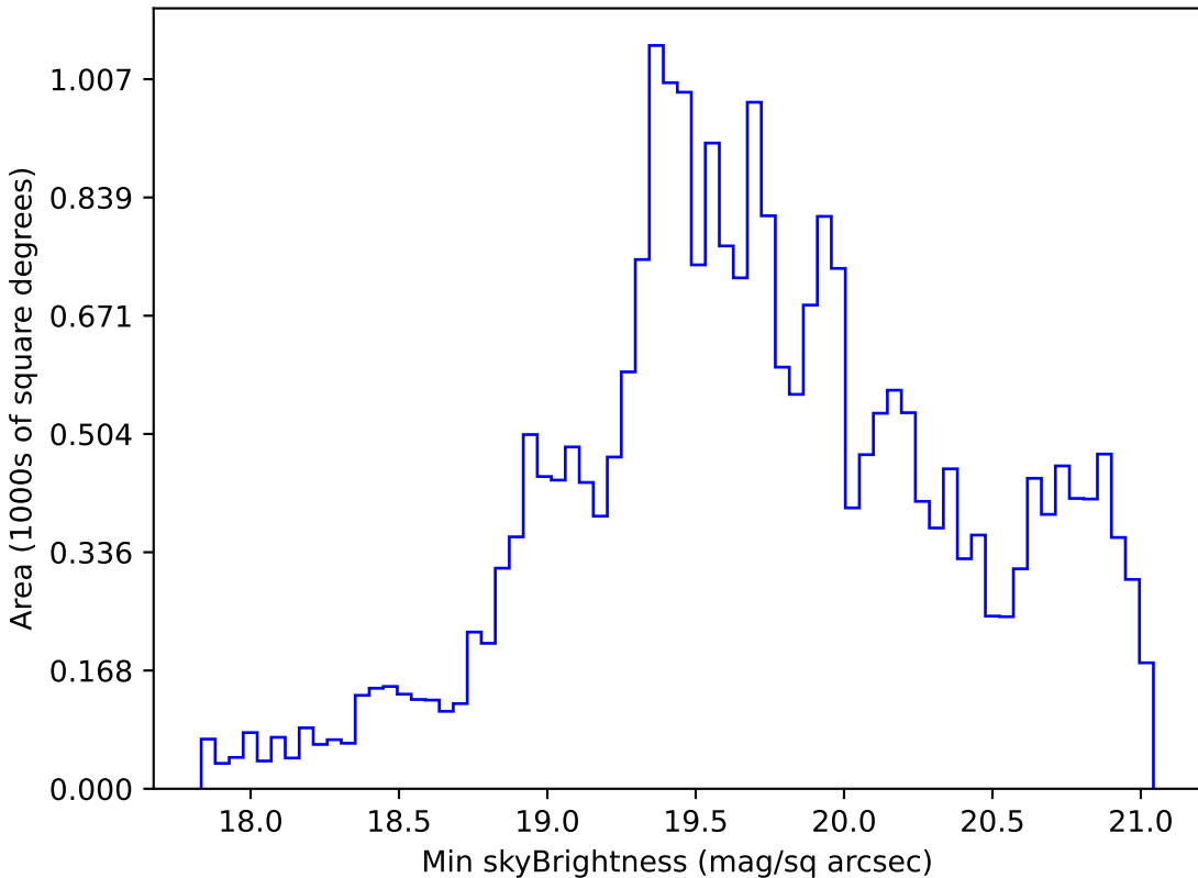
too_10_1v3.4_10yrs Yr 1 r band: Min skyBrightness
