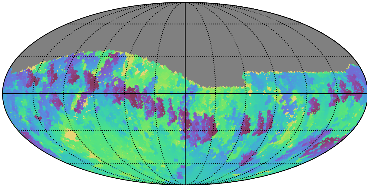
too_10_1v3.4_10yrs Yr 1 i band: Min skyBrightness
