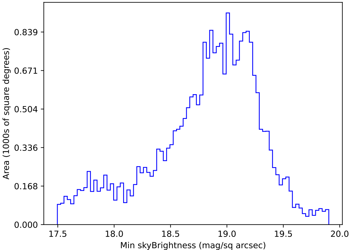
too_10_1v3.4_10yrs Yr 1 i band: Min skyBrightness
