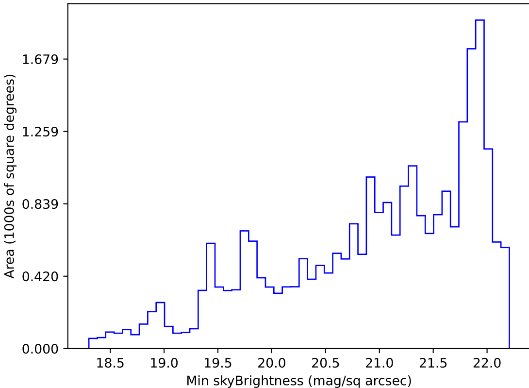
too_10_1v3.4_10yrs Yr 1 g band: Min skyBrightness
