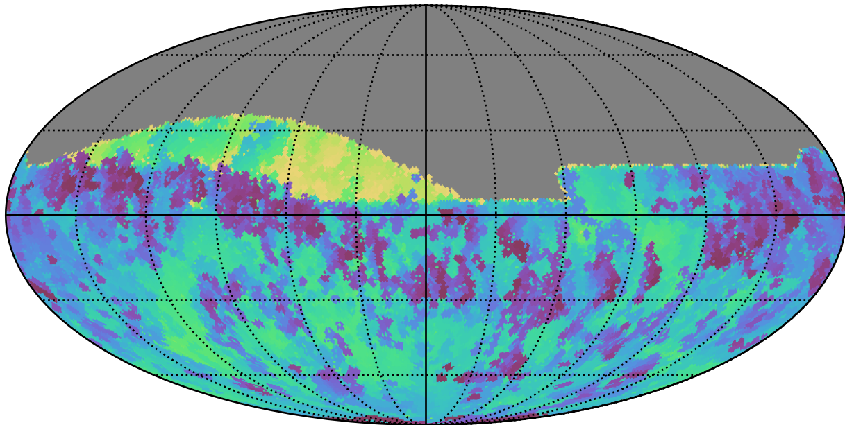
too_10_1v3.4_10yrs Yr 1 all bands: Min skyBrightness
