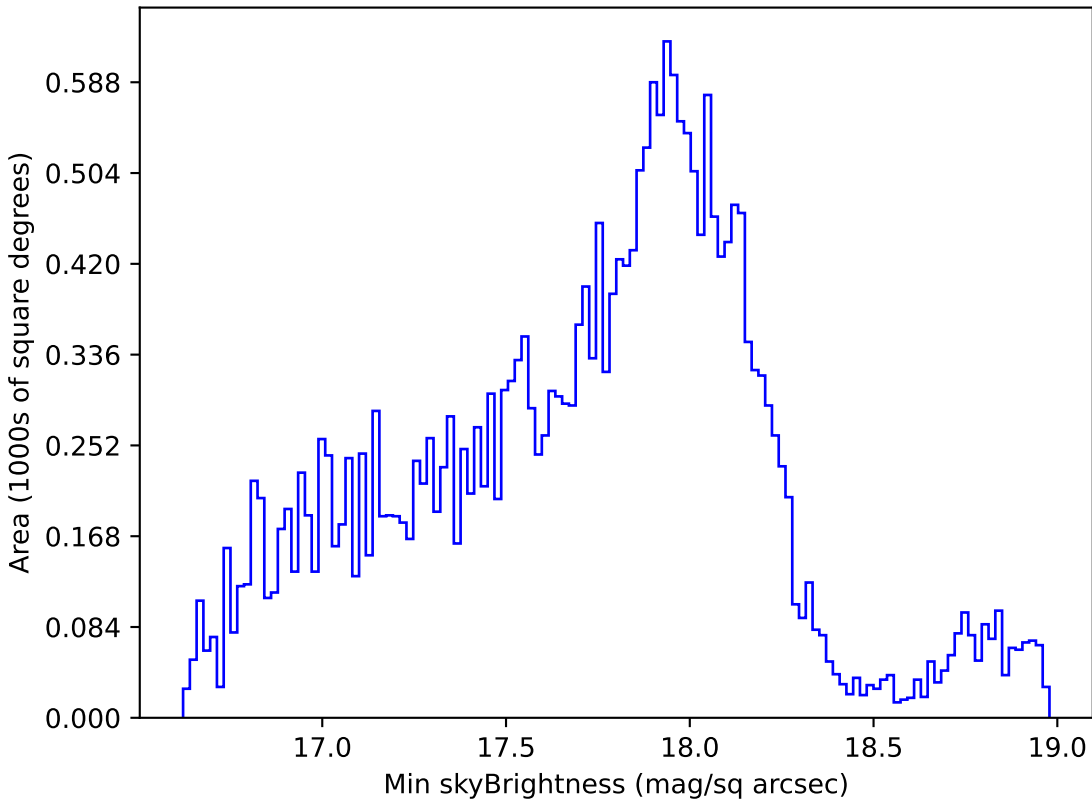
too_10_1v3.4_10yrs Yr 1 all bands: Min skyBrightness
