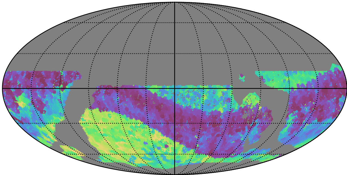
too_10_1v3.4_10yrs WFD z band: Min skyBrightness
