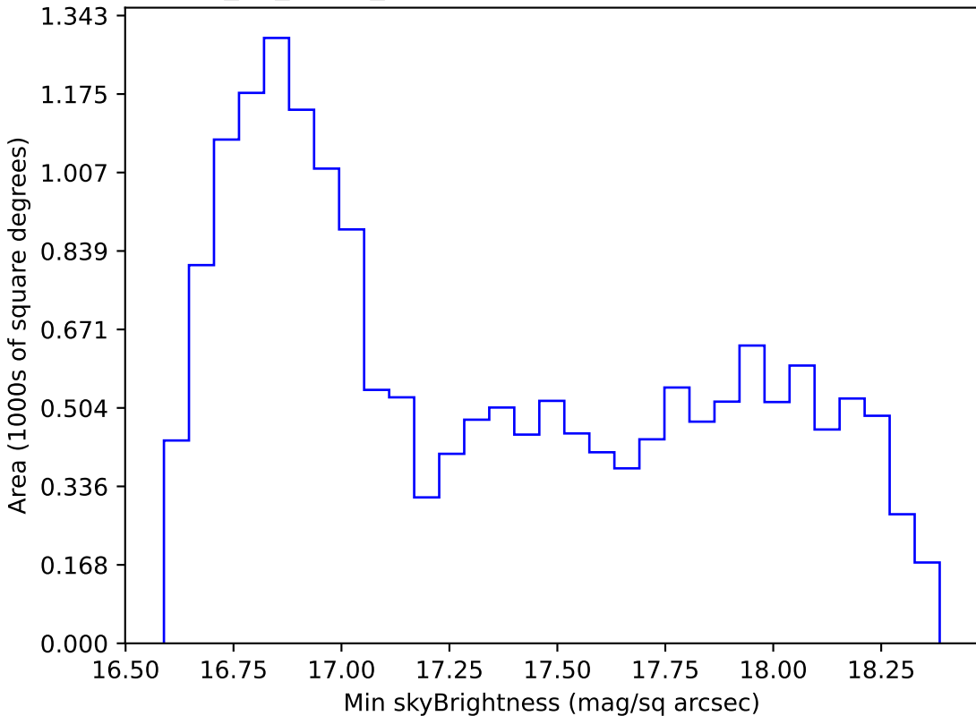
too_10_1v3.4_10yrs WFD z band: Min skyBrightness
