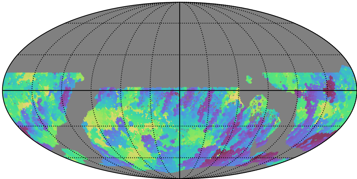
too_10_1v3.4_10yrs WFD r band: Min skyBrightness
