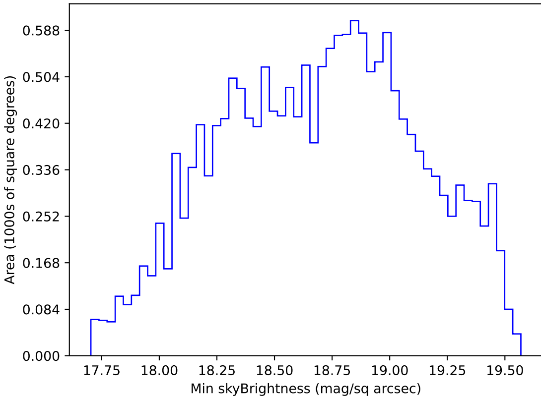
too_10_1v3.4_10yrs WFD r band: Min skyBrightness
