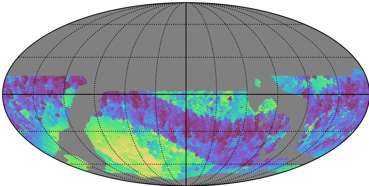
too_10_1v3.4_10yrs WFD i band: Min skyBrightness
